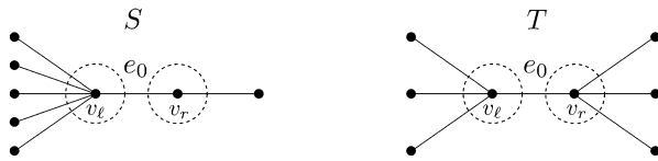
(a) Preferential attachment. The degrees of v_\ell and v_r are unbalanced in S but balanced in T , and this likely remains the case as the trees grow according to preferential attachment. This is at the root of why S and T are distinguishable as seed trees in the preferential attachment model.
