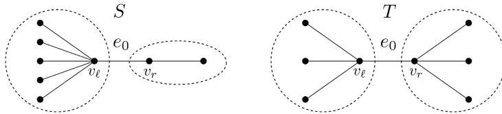
(b) Uniform attachment. The sizes of the subtrees under v_\ell and v_r are unbalanced in S but balanced in T , and this likely remains the case as the trees grow according to uniform attachment. This is at the root of why S and T are distinguishable as seed trees in the uniform attachment model.
